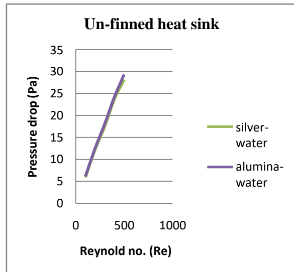
Fig.11: Variation of pressure drop with Re with different Nano-fluid for Un-finned heat sink.
