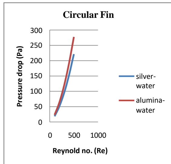
Fig.10: Variation of pressure drop with Re with different Nano-fluid for Circular-finned heat sink.
