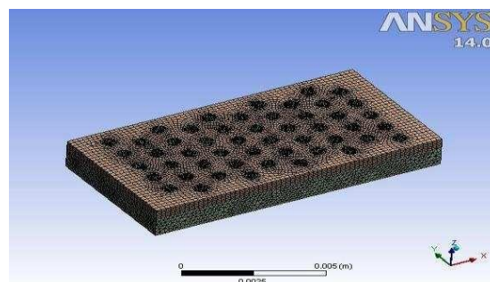
Fig. 2: Meshing of circular finned MPFHS
