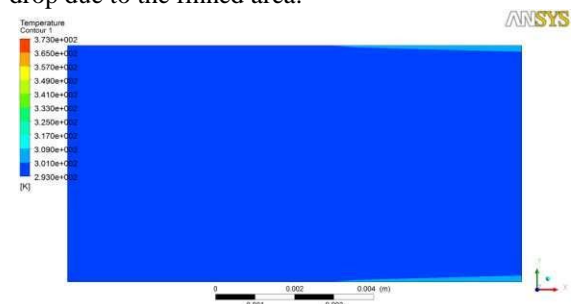
Fig. 7: Static temperature contour of un-finned MPFHS (at Re=500).
