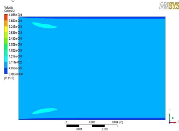
Fig. 5: Velocity contour of Un-finned MPFHS (at Re=100).
