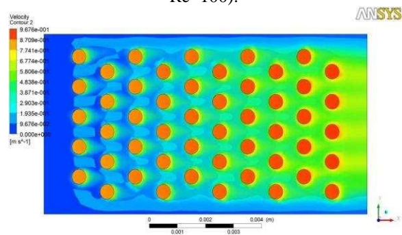
Fig. 6: Velocity contour of circular-finned MPFHS (at Re=100).
